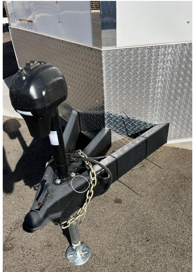
60" Tipple Tube Tongue 2-5/16" coupler Electric optional
